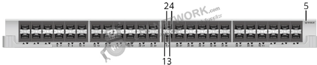
Figure 2 show the indicators on the ES1D2X48SX2S panel.
