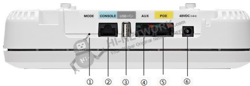
Figure 3 shows AIR-AP1852I Ports and Connections.
